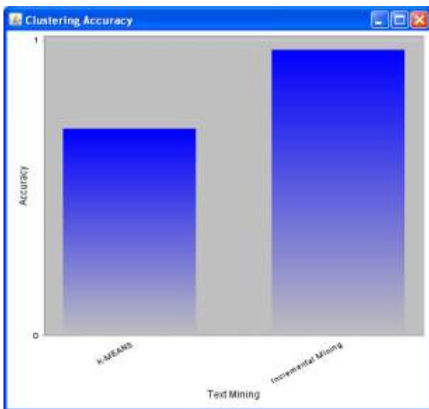
Figure 2: Clustering Accuracy
