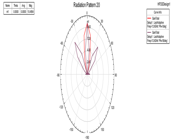
Fig.7 Radiation Pattern for Circular patch antenna
