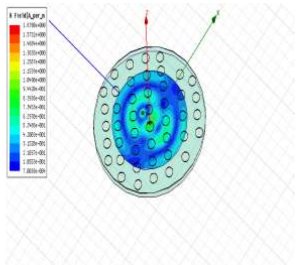
Fig 8. Magnetic Field distribution for circular patch antenna
