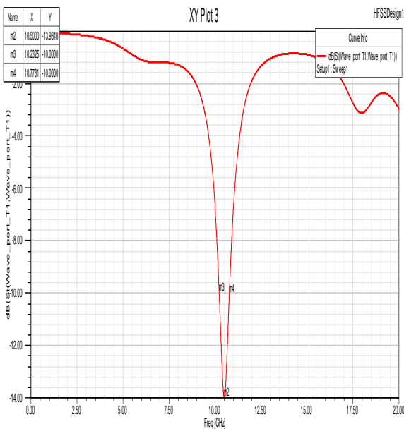
Fig 2. Frequency Vs return loss plot for
