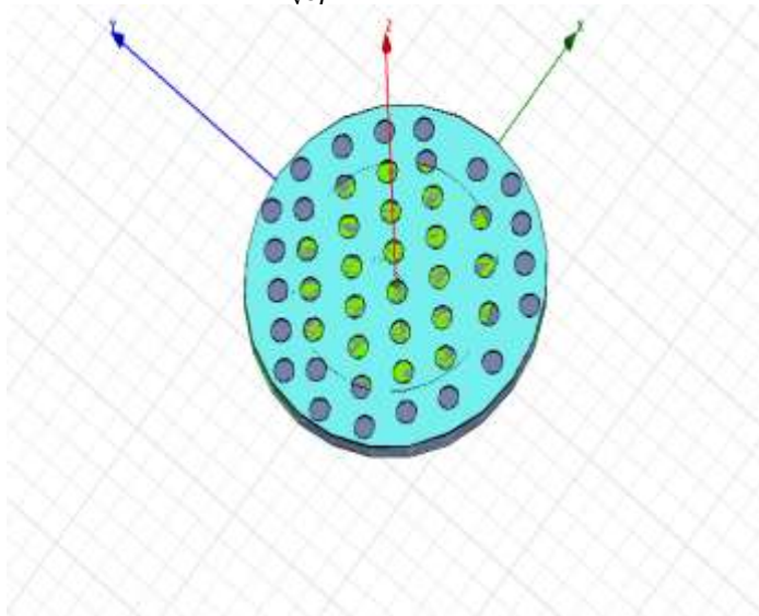
Fig. 5 Top and Side view of Circular patch antenna
