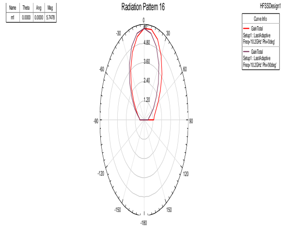
Fig 3. Radiation Pattern for rectangular patch antenna
