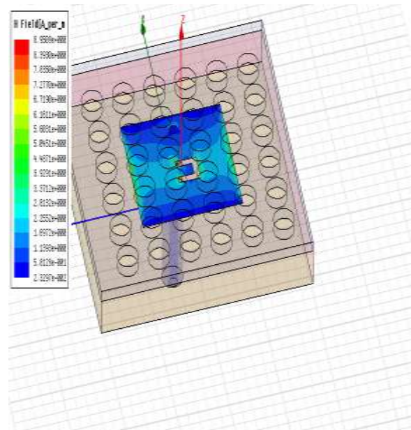
Fig 4. Magnetic Field distribution for rectangular patch antenna
