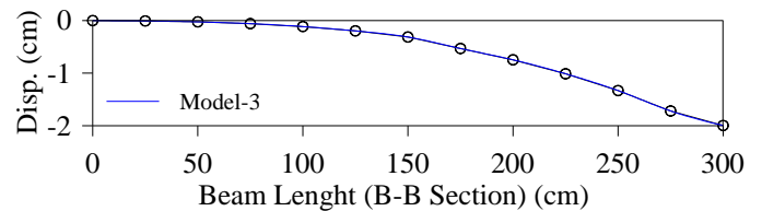
Fig. 8: Vertical displacements on the beam for Model-3
