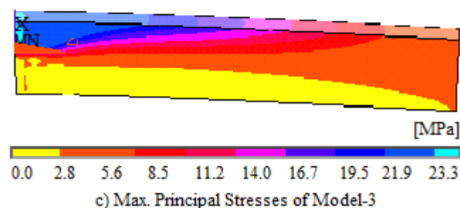
Fig. 12: Maximum principal stresses contour diagrams
