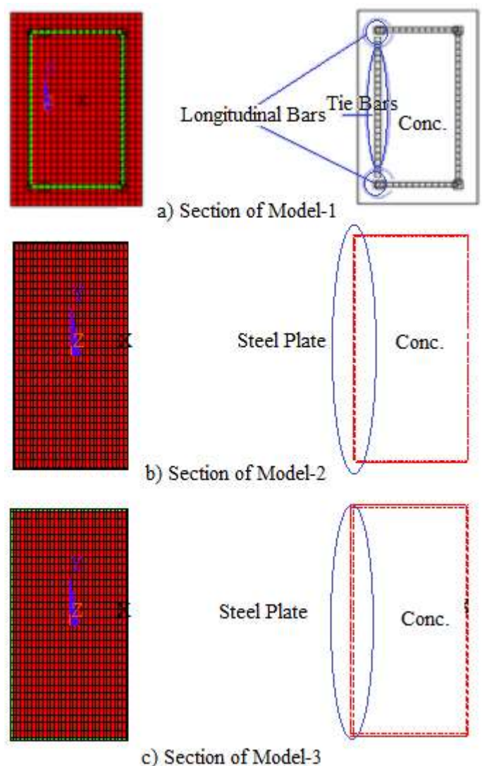
Fig.2: The sections of the beam models
