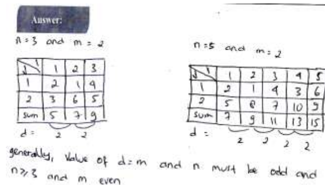
Figure 6: Reasoning effectively
