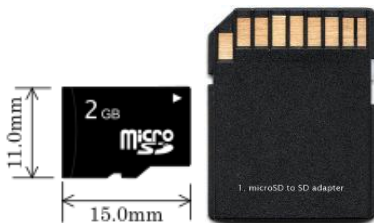
Fig. 5. Micro SD card and Adapter
