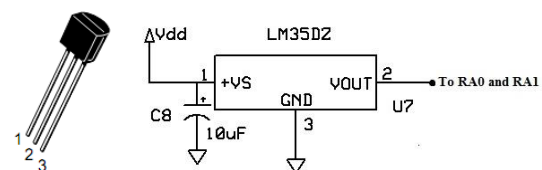
Fig. 3. Pin Configuration and Connection diagram of LM35DZ
