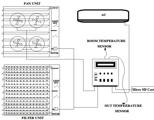
Fig. 1. Total Free Cooling Unit (FCU) system .
