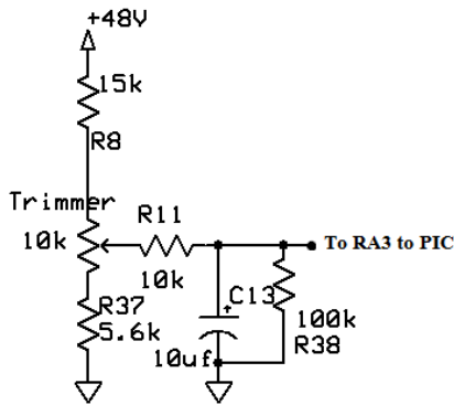
Fig. 4. Battery Voltage monitoring Section
