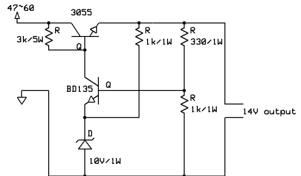
Fig. 2. Power supply section
