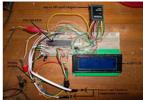
Fig. 10. Practical setup of the Controller Unit
