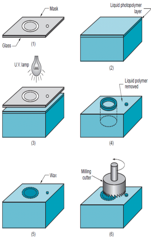
Figure 5: Solid ground curing process for each layer :
