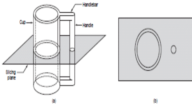
Figure 2: Conversion of a solid model of an object into layers.
