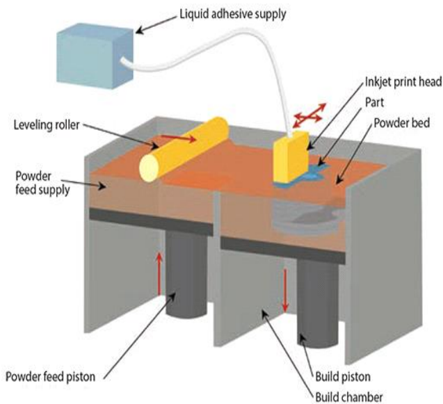
Figure 10: Three Dimensional Printing
