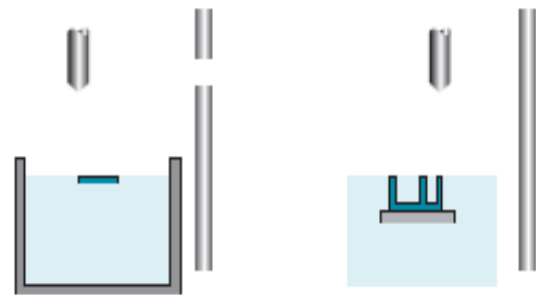
Figure 3: Stereolithography
