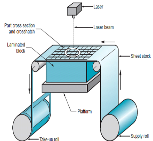
Figure 7: Laminated-object manufacturing
