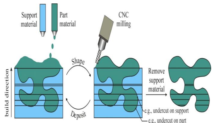
Figure 6: Droplet Deposition Manufacturing
