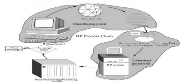
Figure 1: Principle and Process of Rapid Prototyping
