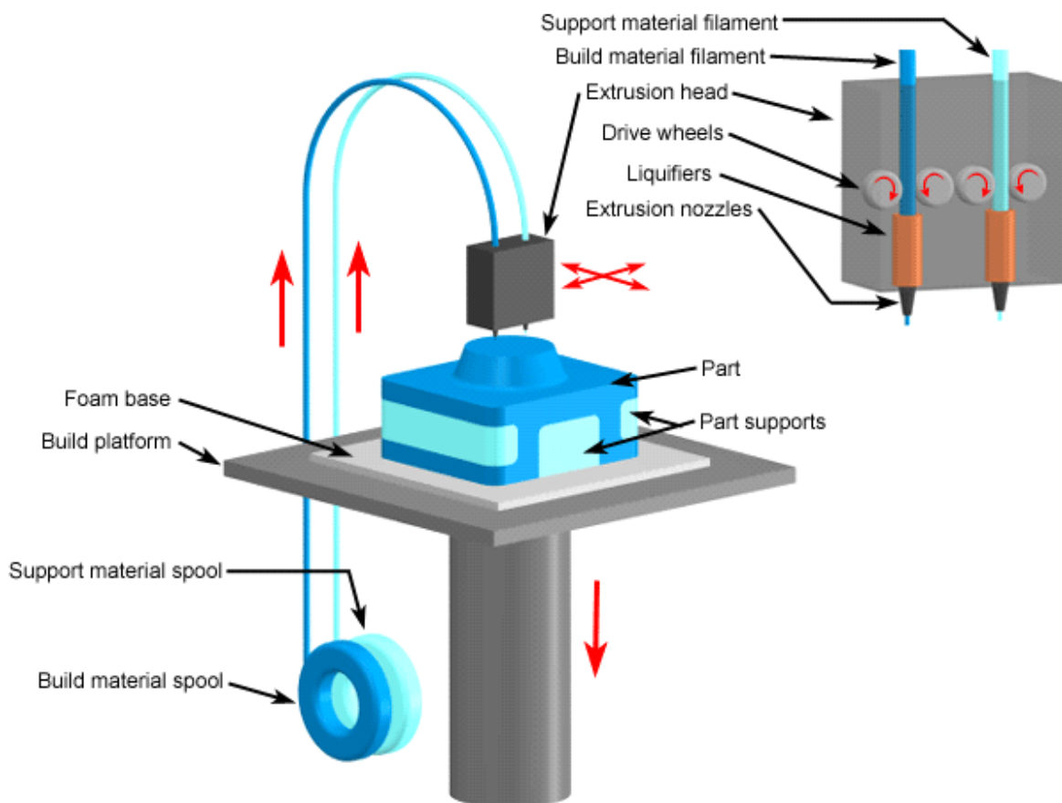
Figure 8: Fused Deposition Modelling
