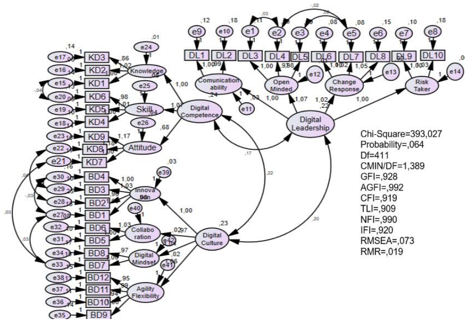
Figure 1. Model_CFA Construct diagram
