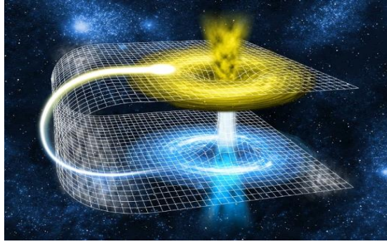
Picture 5: A kind of connection between 2 black holes
