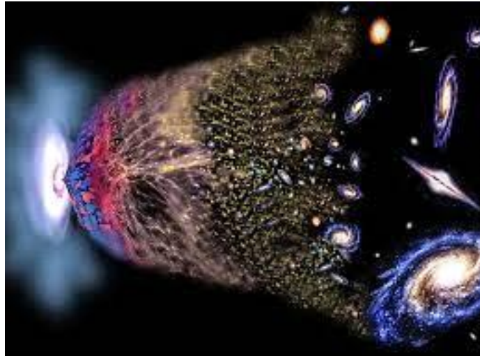
Picture 1: first big bang
