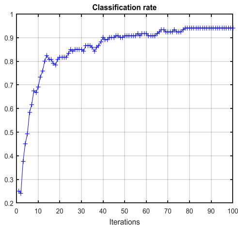
Fig 5 Classification rate for LBP and e-PCA, reaching and converging to 94.7 at around 80iterations
