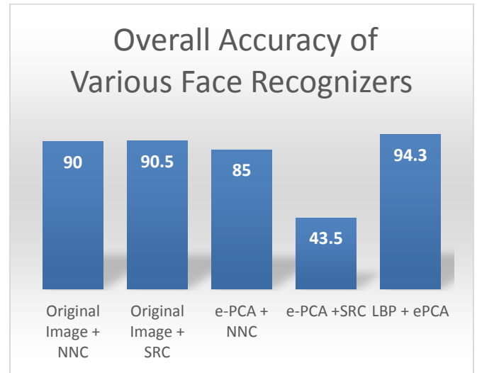
Fig 6 Overall Accuracy of Various Algorithms Compared
